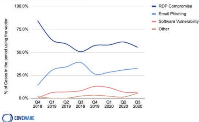
Ransomware Attack Vectors
