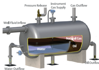
Typical Separator
