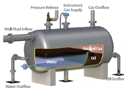
Typical Separator
